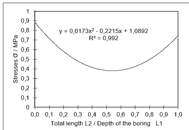
Figure 3 The bushing contact surface stresses dependence by the L2 / L1 ratio
