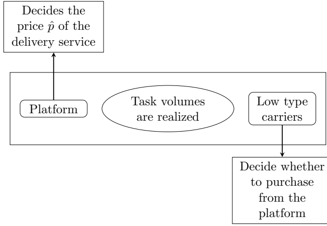
Figure 2: The sequence of decisions under the capacity sharing platform business model capacity can successfully sell it. However, if the demand is less than the supply, then only a subset of these carriers can sell their remaining capacity. In this situation, the platform will randomly distribute the tasks with an equal probability to the carriers willing to sell their remaining capacity.
