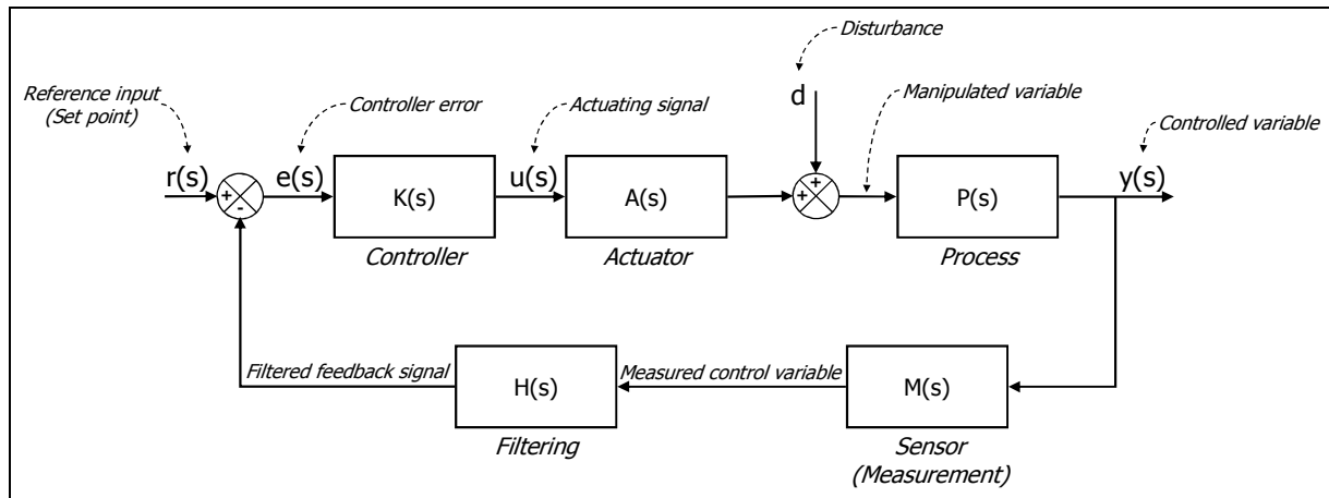
Figure 7: Classical control loop
