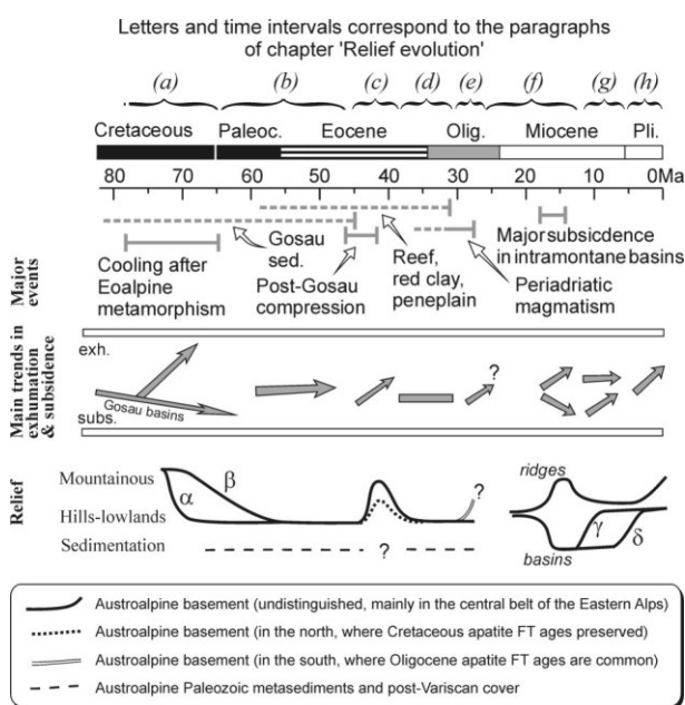
FIGURE 7: Summary of the major structural events, sedimentation periods, dominant trends in exhumation or subsidence, and the deduced relief evolution of the eastern part of Eastern Alps. Explanation of relief evolution paths \alpha , \beta , \gamma and \delta is in the text.
