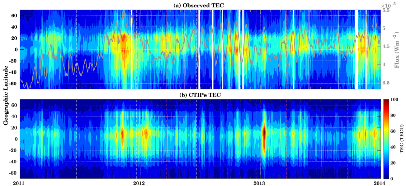
Figure 3. Latitudinal variation of (a) observed TEC and (b) model-simulated TEC around noon (11:00–13:00 LT) at 15° E longitude. The gray curve in panel (a) represents the SDO EVE-integrated flux (1–120 nm).
