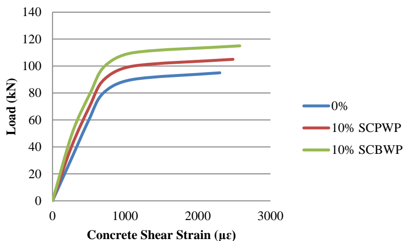
Figure 7. Load-strain curves for beam with full shear reinforcement (SS=100 mm)
