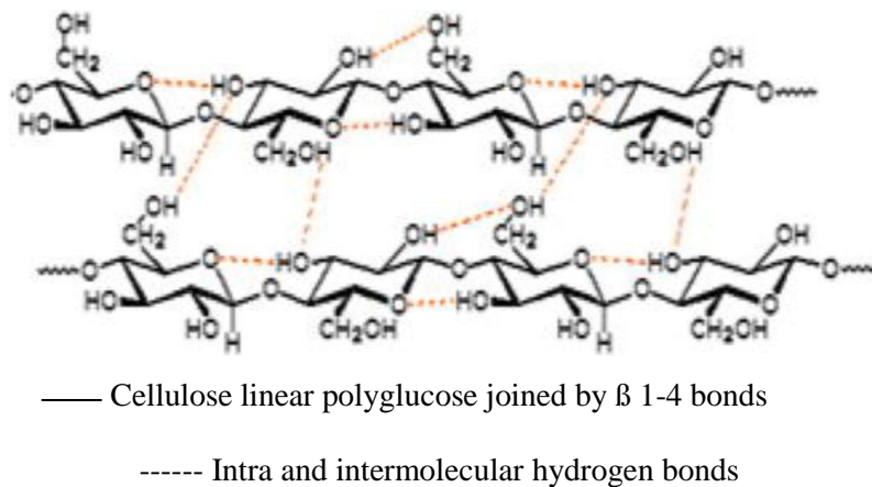
Figure 3. Paper chemical structure (Cellulose hydrogen bond)
