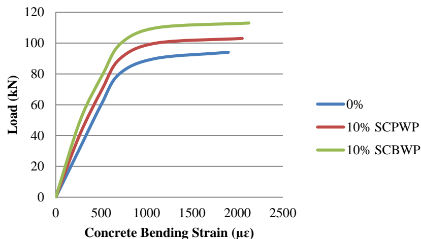
Figure 4. Load-strain curves for beam with full shear reinforcement (SS=100 mm)
