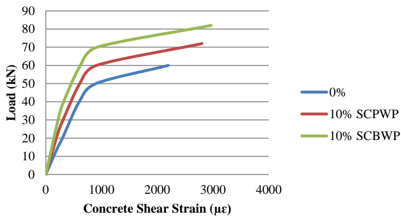
Figure 9. Load-strain curves for beam with reducing shear reinforcement (SS=200 mm)
