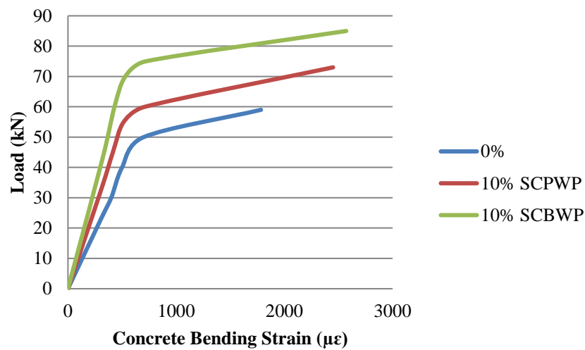
Figure 6. Load-strain curves for beam with reducing shear reinforcement (SS=200 mm)
