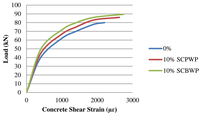
Figure 8. Load-strain curves for beam with reducing shear reinforcement (SS=150 mm)
