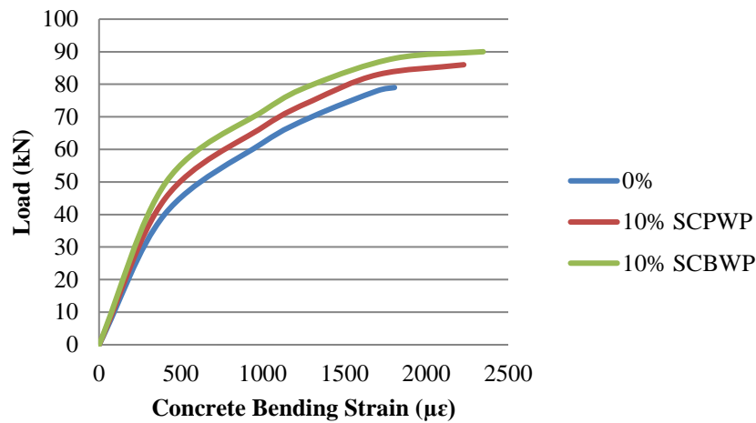
Figure 5. Load-strain curves for beam with reducing shear reinforcement (SS=150 mm)
