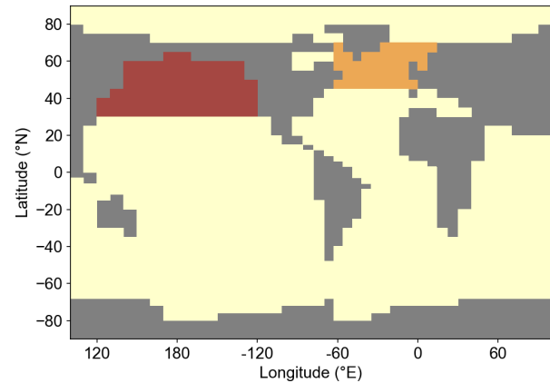
Figure B1. Map depicting regions where freshwater and saltwater perturbations are applied. For the hosing experiments, the freshwater was evenly applied to the North Atlantic (orange). In order to achieve weakened LGM AMOC states, small freshwater fluxes were added to the North Atlantic (orange) and compensated for in the North Pacific (red) by adding the equivalent salt flux to that region.
