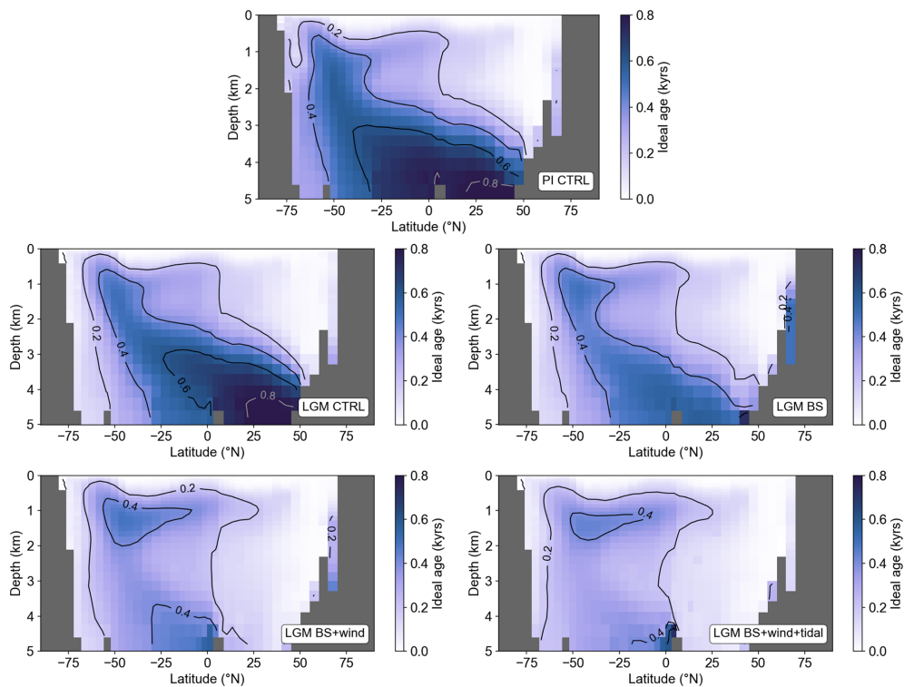
Figure B3. Zonally averaged ideal water ages of the Atlantic for the different model configurations listed in Table 1. Ideal ages are set to zero at the surface and increase in the ocean interior at a rate of 1 yr yr -1 .
