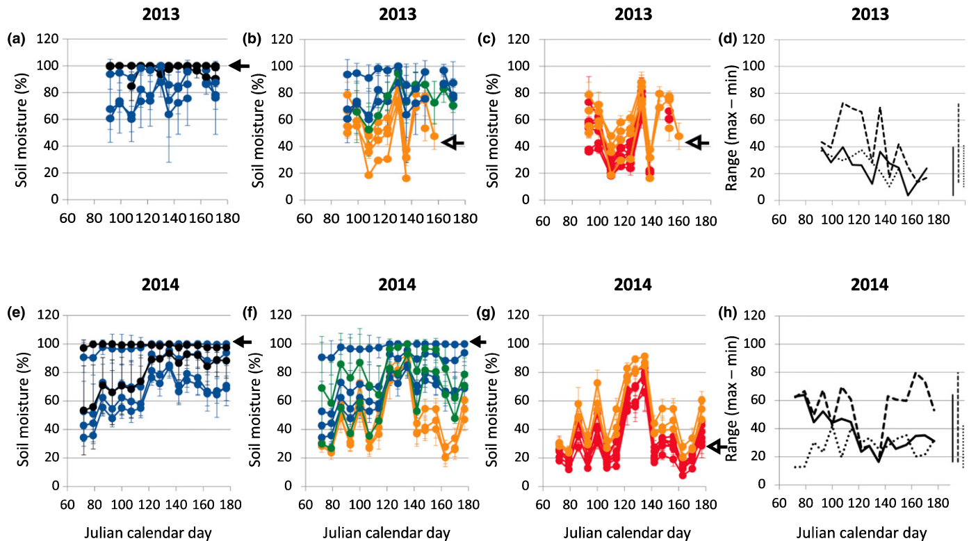
Fig. 3 The mean \pm SD and the range (maximum–minimum) of soil moisture of Cardamine amara , Cardamine hirsuta , and Cardamine flexuosa sites during growing seasons in (a–d) 2013 and (e–h) 2014 measured with a soil moisture sensor at each site ( 3 \leq N \leq 9 per site). (a, e) Mean soil moisture of sites with C. amara . (b, f) Mean soil moisture of sites with C. flexuosa . (c, g) Mean soil moisture of sites with C. hirsuta . In (a–c) and (e–g), the color coding of points corresponds to that in Figs 1, 2, and open and filled arrows indicate the IR5 and KT1 sites, respectively. IR, Irchel; KT, Künsnacht-Tobel. (d, h) The range of soil moisture on census dates and for the entire growing season (vertical bars on the right) for each species; solid, dotted, and finely dotted lines indicate C. amara , C. flexuosa , and C. hirsuta , respectively. In 2013, C. flexuosa did not occur in the wettest site, KT1, inhabited by C. amara (a, filled arrowhead) but appeared in the driest site, IR5, inhabited by C. hirsuta (b, c, open arrowheads). The opposite was the case in 2014 (e–g).
