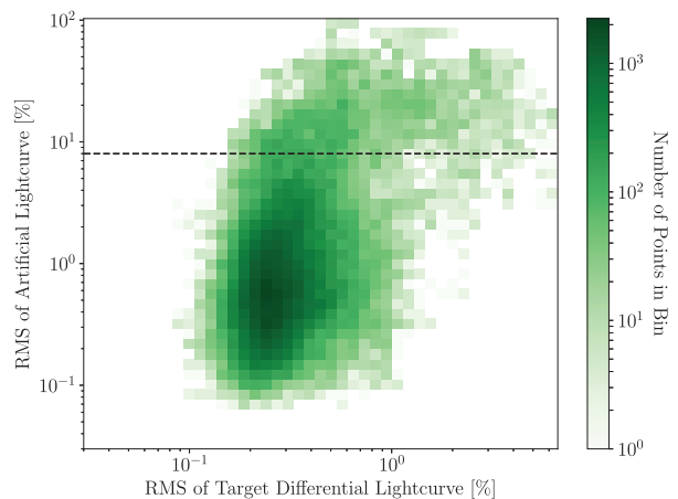
Figure 4. Local rms of unbinned artificial light curves (ALC) against local rms of unbinned target differential light curves for all of Io’s observations since 2019 January 1. For this analysis, there is no water vapour correction or removal of cosmic hits, flares or variability, which may cause a points at low ALC rms but a high target light curve RMS of a few per cent. It is clear there is an much larger variation in quality of the target differential light curves when the local rms of the ALCs exceeds the threshold of \sim 8 per cent, shown by the black dashed line.
