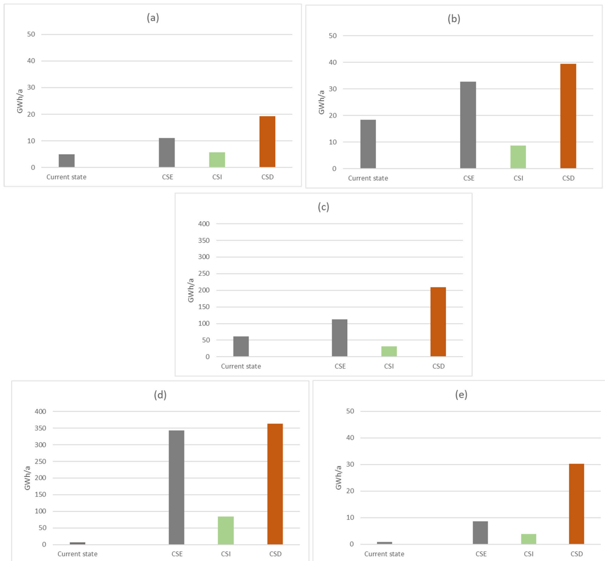
Figure 3. Estimates of energy intensity for water production with the three scenarios ( Current State Extends (CSE) , Current State Improves (CSI) and Current State Deteriorates (CSD) ) for 2030 compared to current energy intensity (2019). Note the difference in magnitude for energy intensity between WSP1 (a), WSP2 (b) & WSP5 (e) and WSP3 (c) & WSP4 (d).
