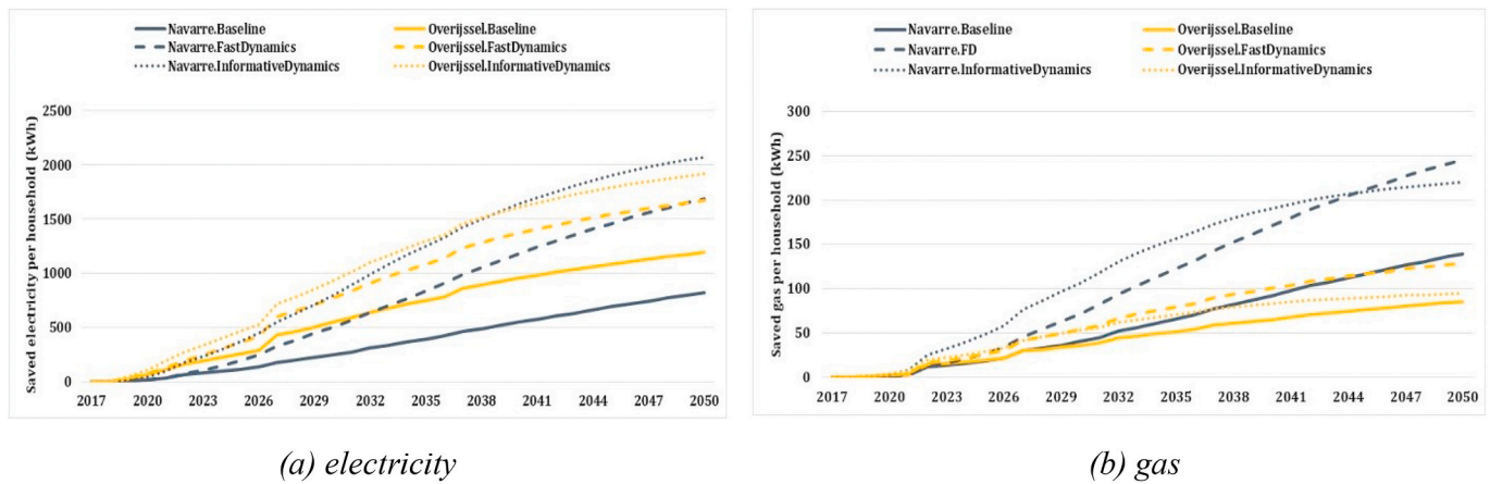
Fig. 5. Saved energy (kWh) per household as a result of investment (I1–I3) under three behavioral scenarios in two EU provinces over 34 years (2017–2050). Source: BENCH-v.3.
