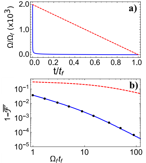
FIG. 3. (a) Transverse field \Omega(t) for the linear ramp (dashed) and FAQUAD (solid) protocols to implement the perceptron gate. (b) Average infidelity 1 - \bar{\mathcal{F}} as a function of the total ramp time t_f , for the two ramp protocols. The FAQUAD process is fitted by \sim c_0 \exp[-c_1(\Omega_f t_f)^{c_2}] , c_0 = 26.838 , c_1 = 6.577 , and c_2 = 0.150 (black circles).
