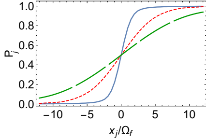
FIG. S3. Quantum perceptron response obtained for FAQUAD passage for different t_f values. Adiabatic passage \Omega_f t_f = 10 (solid), non-adiabatic passages \Omega_f t_f = 1 (short-dashed) and \Omega_f t_f = 0.25 (long-dashed).
