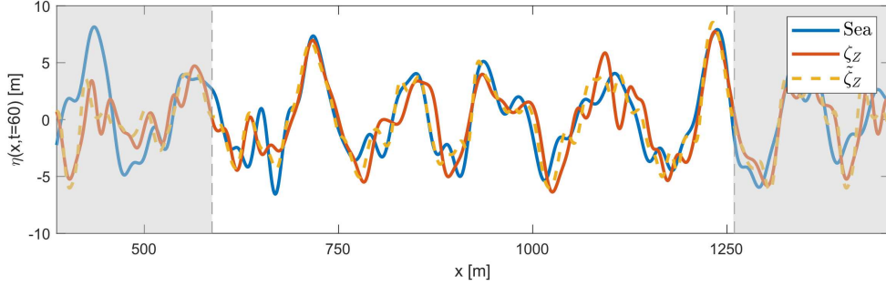
Figure 7: Comparison of a sea (blue curve, containing free and bound modes \eta_1 + \eta_2 ) generated using a JONSWAP spectrum with \epsilon = 0.2 and two forecasts at time t = 60 s. (Red, solid curve) Forecast assuming all modes are free and evolving in time using the Zakharov equation via (19) and (20). (Yellow, dashed curve) Forecast based on identifying the free modes at the measurement time (see red Fourier amplitudes in figure 6, right panel), evolving these in time using the Zakharov equation, and adding the analytical bound modes calculated using (7) at t = 60 s.
