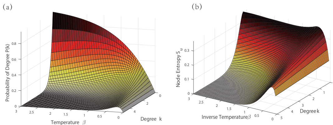
Figure 5. (a) 3D plot of degree probability with different value of degrees k and the inverse temperature \beta ; (b) 3D plot of node entropy with different value of degrees k and the inverse temperature \beta .
