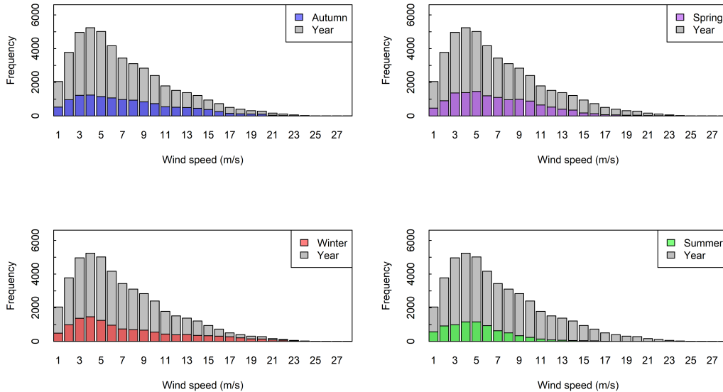
Figure 3: Annual versus seasonal wind speed histograms using 10-minute averaged mean wind speeds
