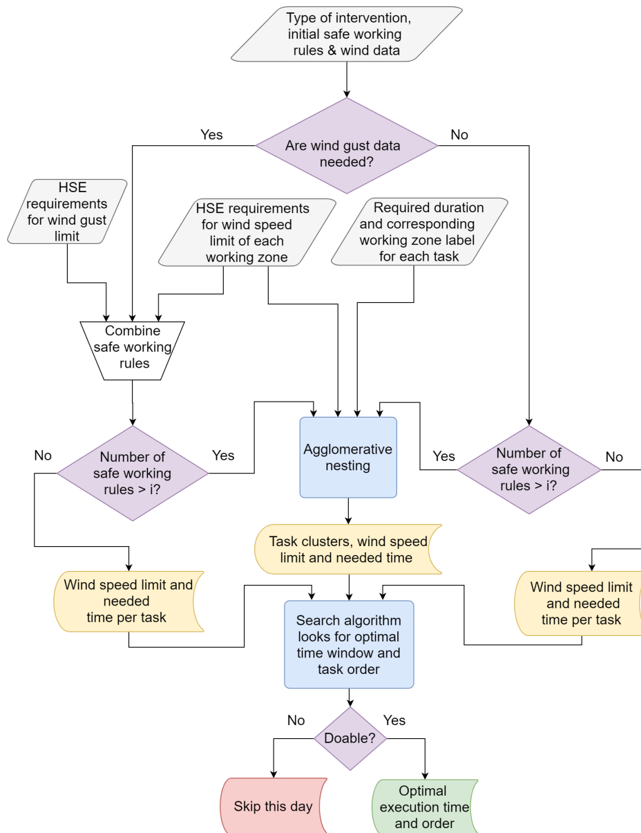
Figure 7: Flowchart of proposed solution, HSE: Health-Safety and Environment regulations
