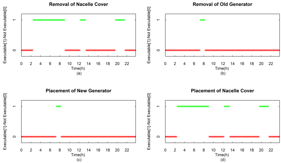
Figure 13: Evaluation of generator replacement when considering dynamic safe working limits due to gust (Summer day).
