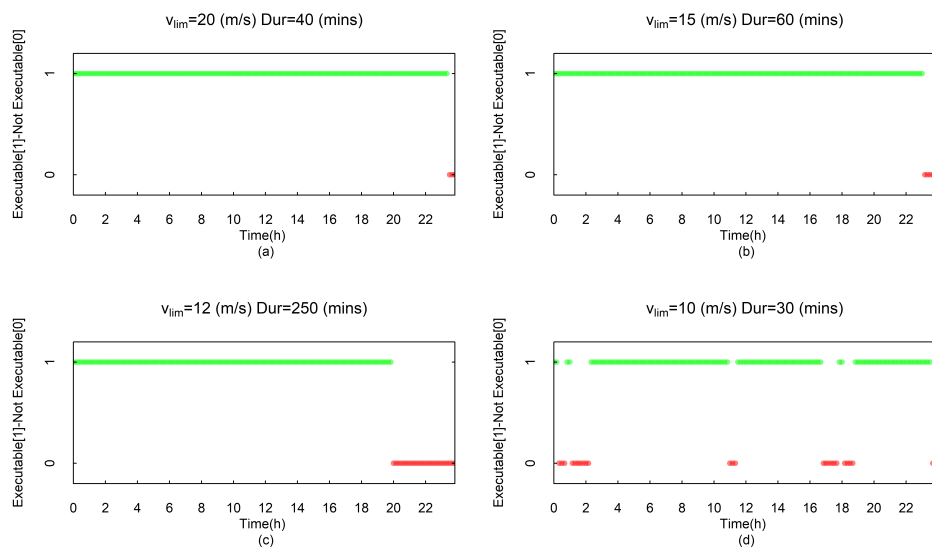
Figure 9: Routine maintenance evaluation with actual input data for the summer day (a) cluster 1, (b) cluster 2 (c) cluster 3 (d) cluster 4
