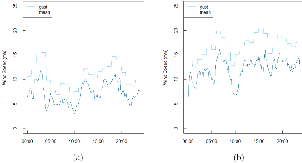
Figure 5: 10-minute mean wind speed and hourly gust during 24 hours. Gust value is repeated for six time steps, since it is only available as one maximum value per hour. (a) Summer day, (b) Autumn day
