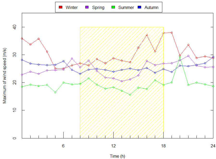
Figure 4: Seasonal wind speed trends as hourly maximums. This figure is obtained calculating the maximums per hour of each day over a season in 2019. The window, which is shaded in yellow represents the day shift from 08:00 to 18:00.
