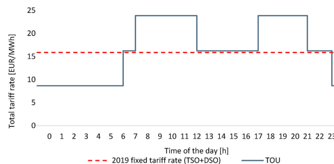
Fig. 6. TOU tariff scheme illustrated.
