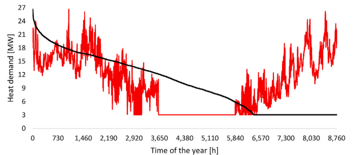
Fig. 4. Heat demand; hourly values and duration curve.
