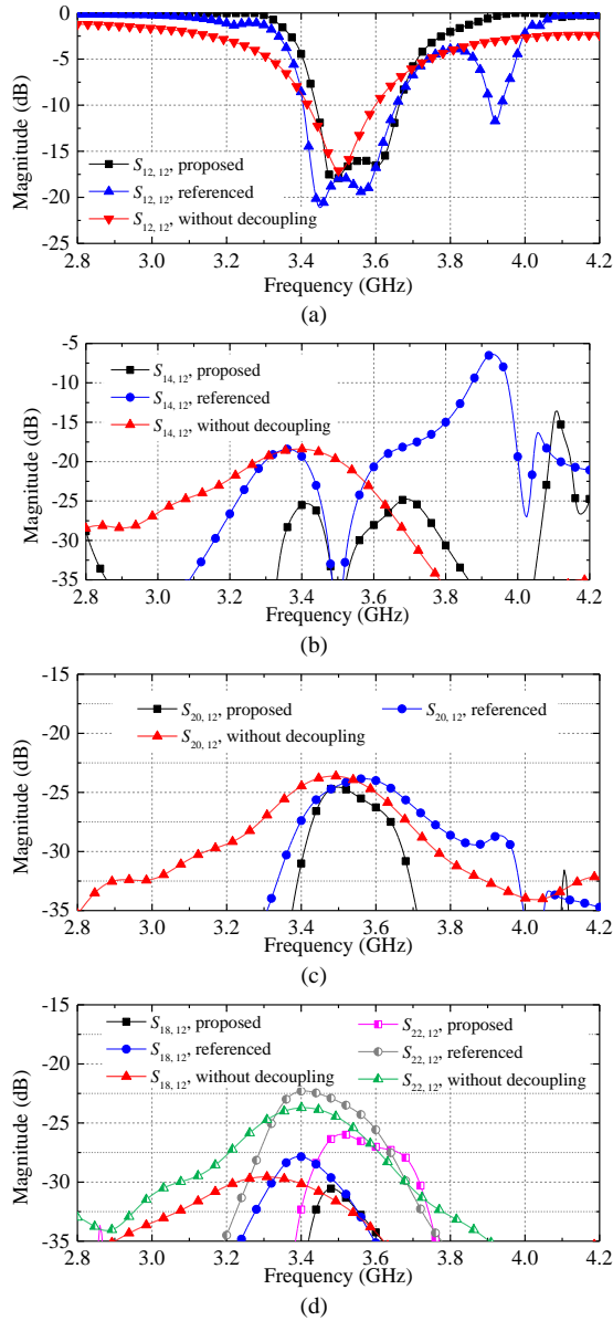
Fig. 11. Calculated mutual coupling of the decoupled 4×4 dual-polarized patch antenna array. (a) S_{12,12'} . (b) S_{14,12'} . (c) S_{20,12'} . (d) S_{18,12'} and S_{22,12'} .
