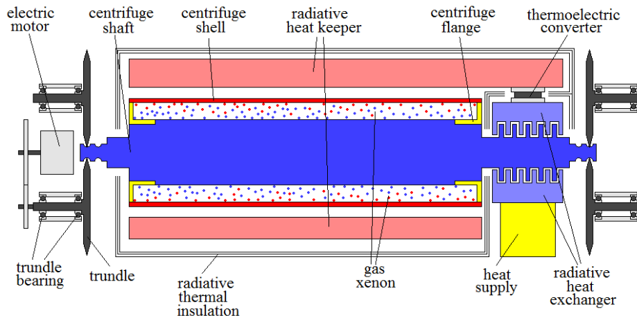
Fig. 3. Schematic section of the setup without background
