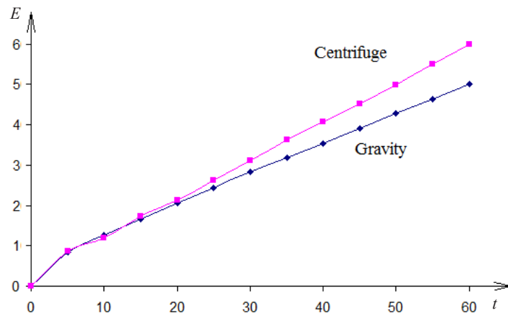
Fig. 2. Molecular trajectories
