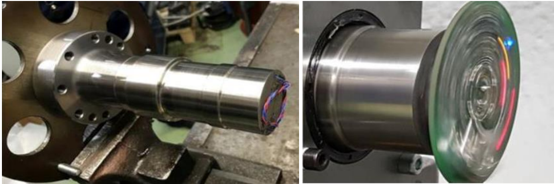
Figure 6. 3D printed metal smart shaft that has an accelerometer inside and wireless data transfer. © 2020 VTT Technical Research Centre of Finland Ltd.
