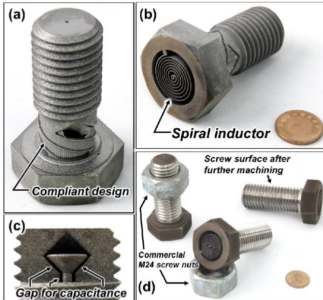
Figure 8. (a) Smart screw with compliant design for feasibility test; (b) closer view of the spiral inductor; (c) cross-sectional view of the gap for capacitance; (d) pilot production result of real-scale smart M24 screws with commercial screw nuts threaded [26]. © 2017 IEEE 6
