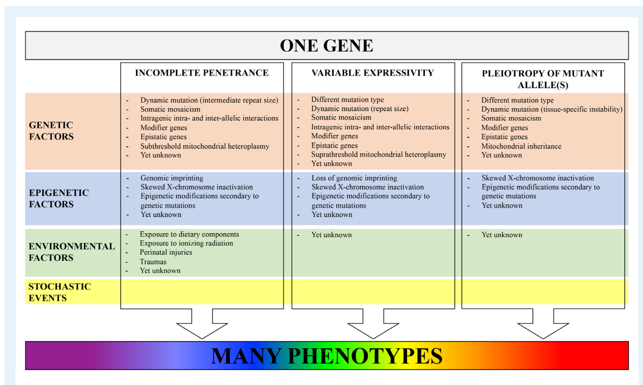
FIG. 2. Overview of genetic and nongenetic (epigenetic, environmental) factors underpinning incomplete penetrance, variable expressivity and pleiotropy of mutant allele(s). Stochastic (ie, random) events might act at all levels and further contribute to phenotypic heterogeneity.
