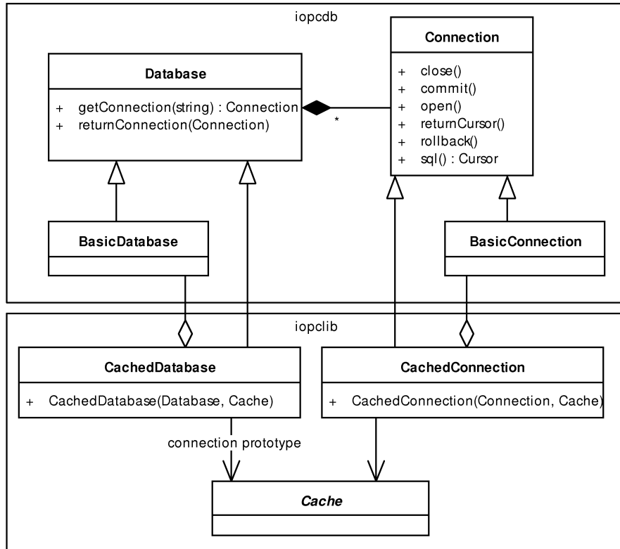
Figure 5.3: Using the decorator pattern
