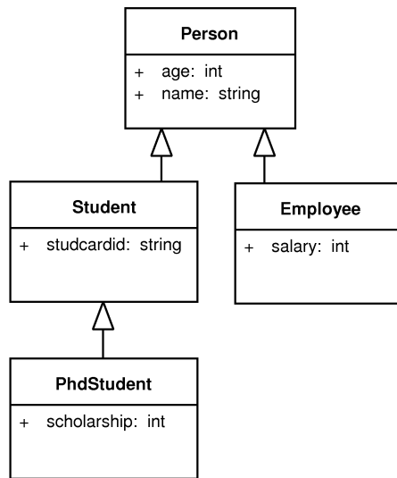
Figure 2.1: Example class hierarchy
