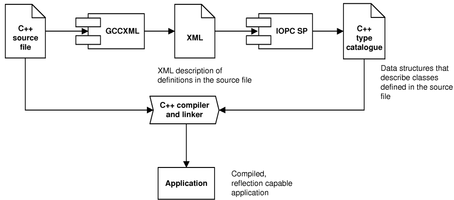
Figure 4.1: Reflection using the GCCXML
