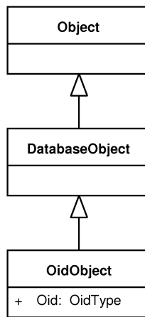
Figure 4.2: IOPC 2 base classes
