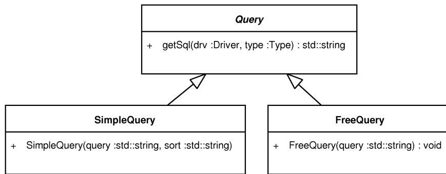
Figure 5.14: The Query classes
