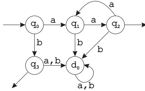
Figure 1.2: Deterministic finite automaton.
