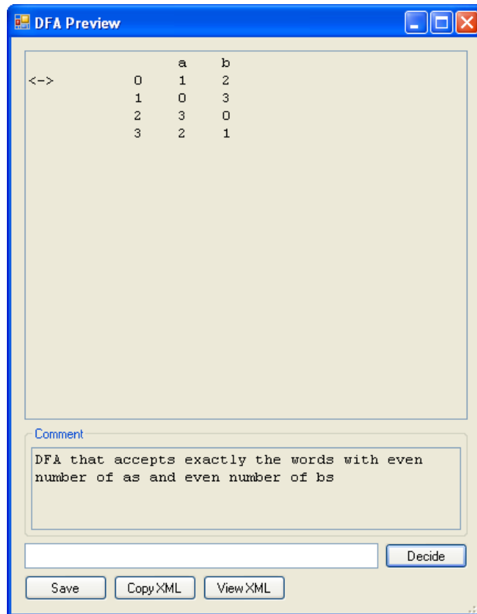
Figure 4.3: DFA Preview form.
