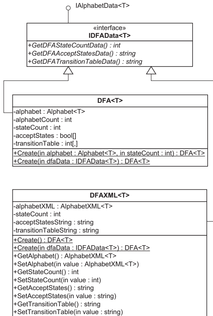
Figure 3.13: DFAXML<T> Class Diagram.
