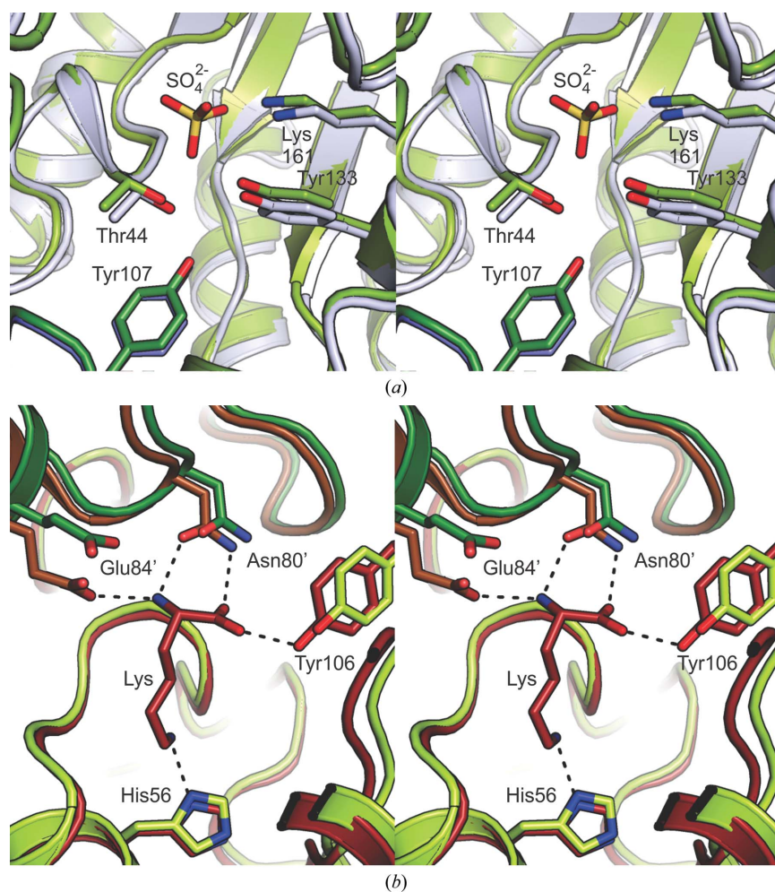
Figure 4 (a) Stereo figure showing the active site of M. fumariolicum SolV (shades of green) superimposed with that of E. coli DapA (light blue/grey). A sulfate (or phosphate; see text) ion is bound in the active site. The residues of the catalytic triad, as well as the catalytic lysine, superimpose closely. (b) Stereo figure showing the putative allosteric pocket in M. fumariolicum SolV (shades of green) superimposed with that in the lysine-inhibited C. jejuni DapA structure (dark red/brown). The residues interacting with the allosteric lysine (Lys) in the C. jejuni structure are conserved in M. fumariolicum SolV DapA, including His56, which is believed to be diagnostic for allosteric regulation. Residues from an adjacent subunit are marked with an apostrophe.
