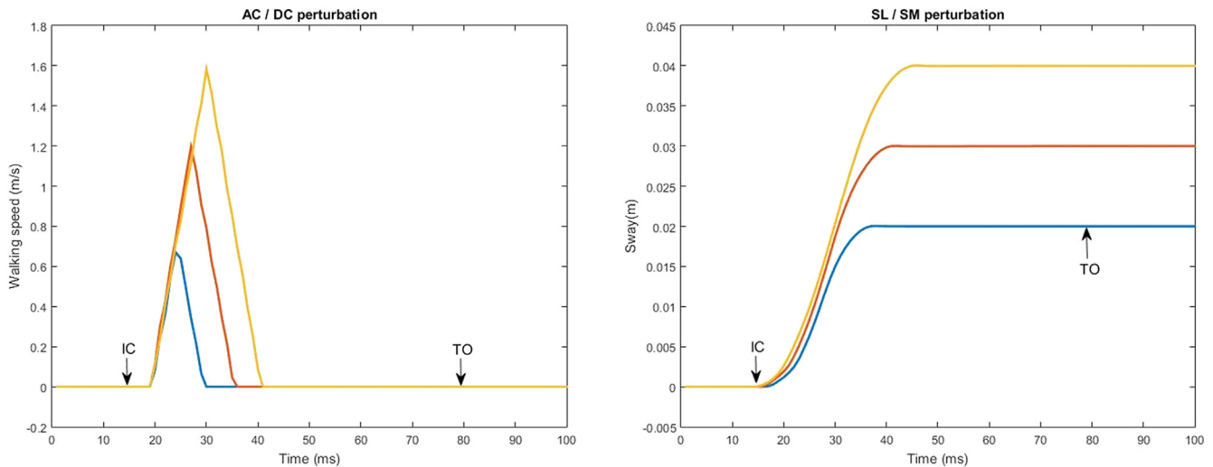
Fig. 2. Specifications of the perturbation types and intensities applied to the subject. Intensity 1 is the blue line, intensity 2 the red line and intensity 3 the yellow line. IC: initial contact, TO: toe off, AC: acceleration of one belt, DC: deceleration of one belt, SL: sway lateral and SM: sway medial.
