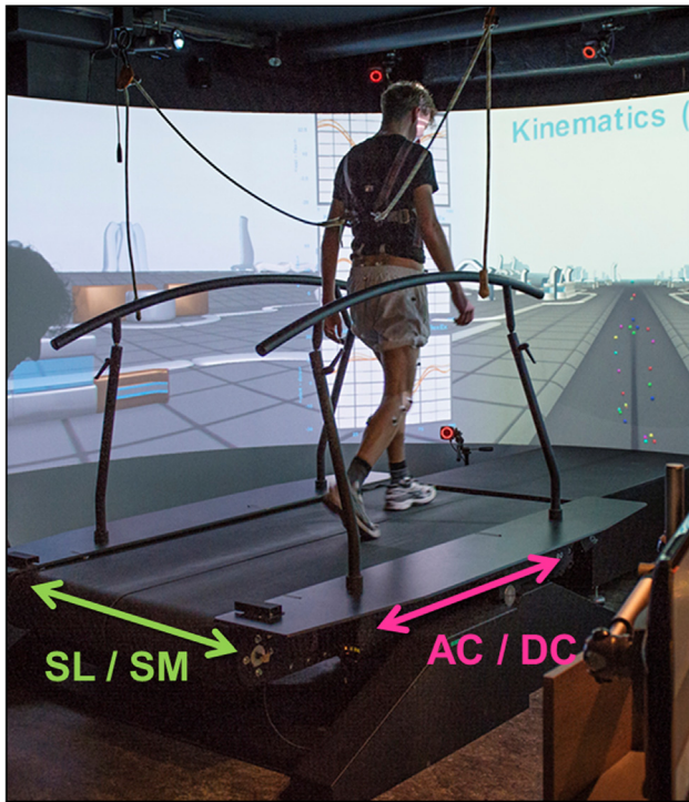
Fig. 1. Overview of the measurement setup and the four perturbation types that can be applied by the GRAIL system. AC: acceleration of one belt, DC: deceleration of one belt, SL: sway lateral and SM: sway medial. Sway Lateral was defined as a sway to the left if the affected leg was left and a sway to the right if the affected leg was right.
