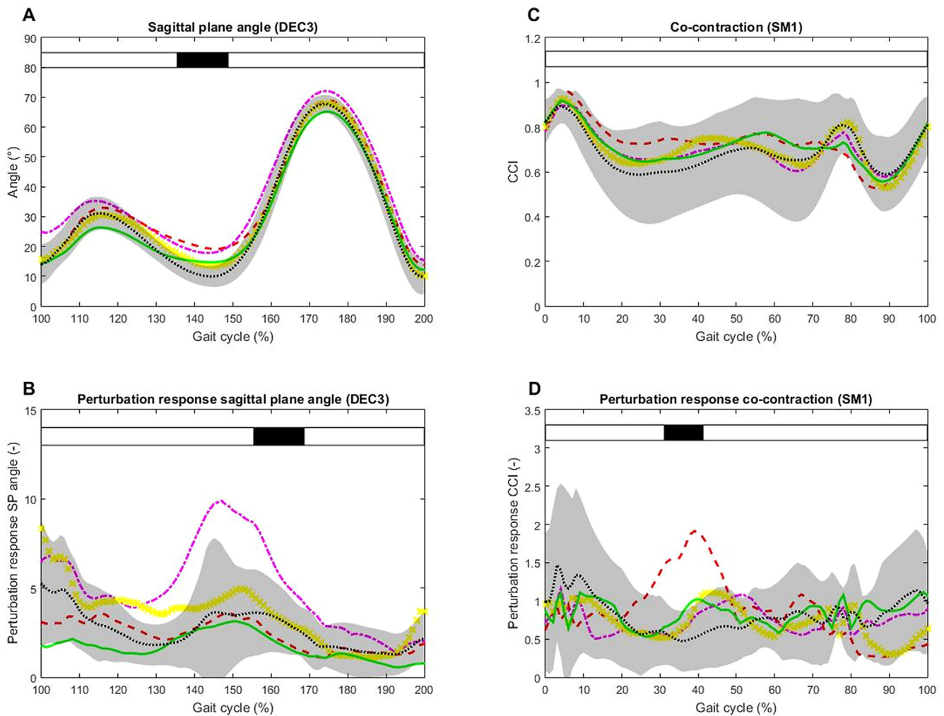
Fig. 5. The sagittal plane angles (5A) and the corresponding perturbation responses (5B) of the subgroups and controls during the stride after the DEC3 perturbation. Furthermore, the co-contraction indices (5C, quadriceps vs. hamstrings) and the corresponding perturbation responses of the co-contraction indices of the subgroups and controls during the perturbed stride of the SM1 perturbation. The subgroups were moderate KOA-I group (magenta, dash-dot line), severe KOA-I group (red, dashed line), moderate KOA-S group (yellow, line of crosses), severe KOA-S group (green, solid line) and healthy control group perturbed (black, dotted line). The line represents the mean pattern of the group and the shaded area represents the standard deviation of the patterns of the control group. Rectangle above graph shows significant differences (black) or not (white) between all groups following from the SPM results.
