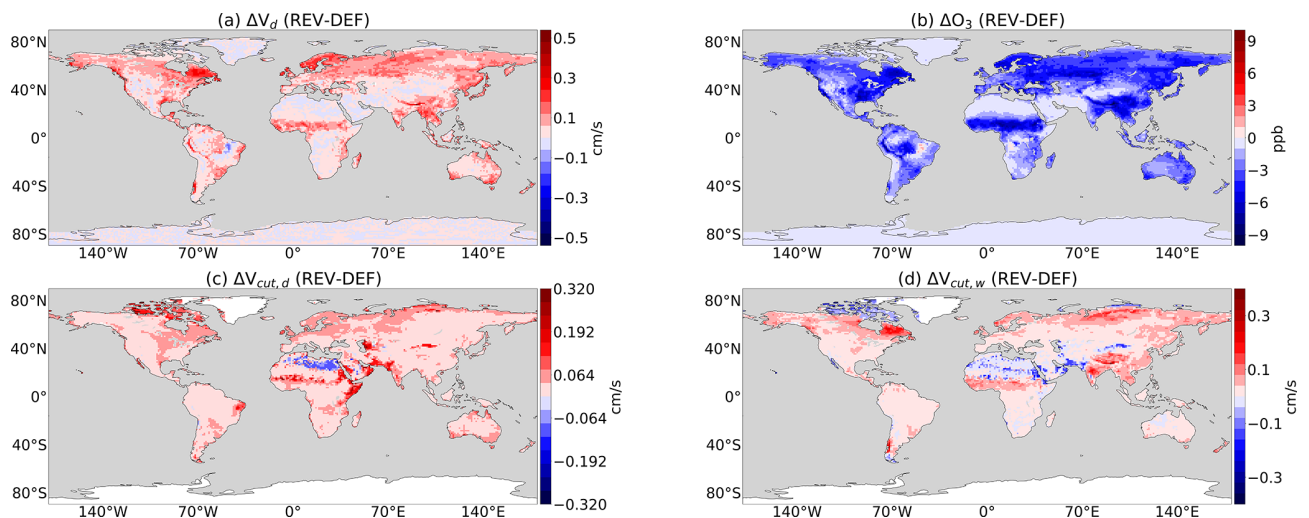
Figure 7. Multiyear (2010–2015) mean absolute changes in boreal summer: i.e. difference between the revised and default scheme (REV – DEF).
