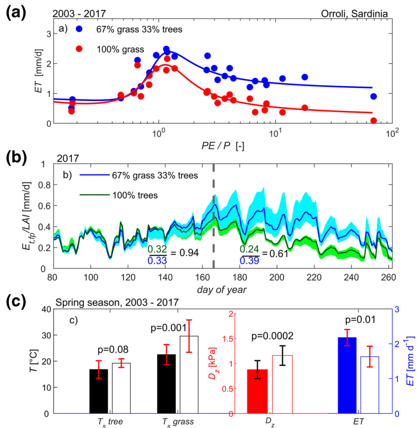
Figure 7. Comparison between the actual ecosystem and land cover change scenarios: (a) evapotranspiration ( ET ) versus dryness index (potential evaporation/precipitation, PE/P ) for the actual ecosystem (67% pasture and 33% tree clumps), and for a hypothetical scenario of 100% pasture without the contribution of tree roots-induced hydraulic redistribution (HR). (b) Predicted tree transpiration at the footprint scale per unit of leaf area index ( E_{t_{fp}}/LAI ) for the actual ecosystem, and for a 100% tree cover scenario. Values in color represent the means for the season for each scenario, and the ratio represent the impact of eliminating HR from the prediction. The shaded areas around the mean bound the 5th and 95th percentiles of the ensemble of predictions generated with the Monte Carlo simulation framework. (c) Observed mean surface temperature ( T_s ) of tree and grass canopies, daytime, day-length normalized vapor pressure deficit ( D_z ), and evapotranspiration ( ET ) for typical ( n = 7 , filled bar) and dry ( n = 2 , unfilled bar) spring seasons (error bars are 1 standard deviations. Note: six incomplete spring time series and an unusually wet spring were excluded). Due to small sample size of dry springs, one sample t-test was used to assess the difference between the mean of the two dry years and the population of typical years.
