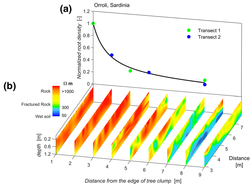
Figure 3. (a) Normalized density of transport roots along 7 m transect from the edge of two tree clumps. (b) inverse model electrical resistivity (in Ohm m) tomography (ERT) images, indicating rock fractures and soil pockets in the subsurface layer (0.2–1.2 m) in transects perpendicular to a root trench at 1 m intervals from the edge of a tree clump.
