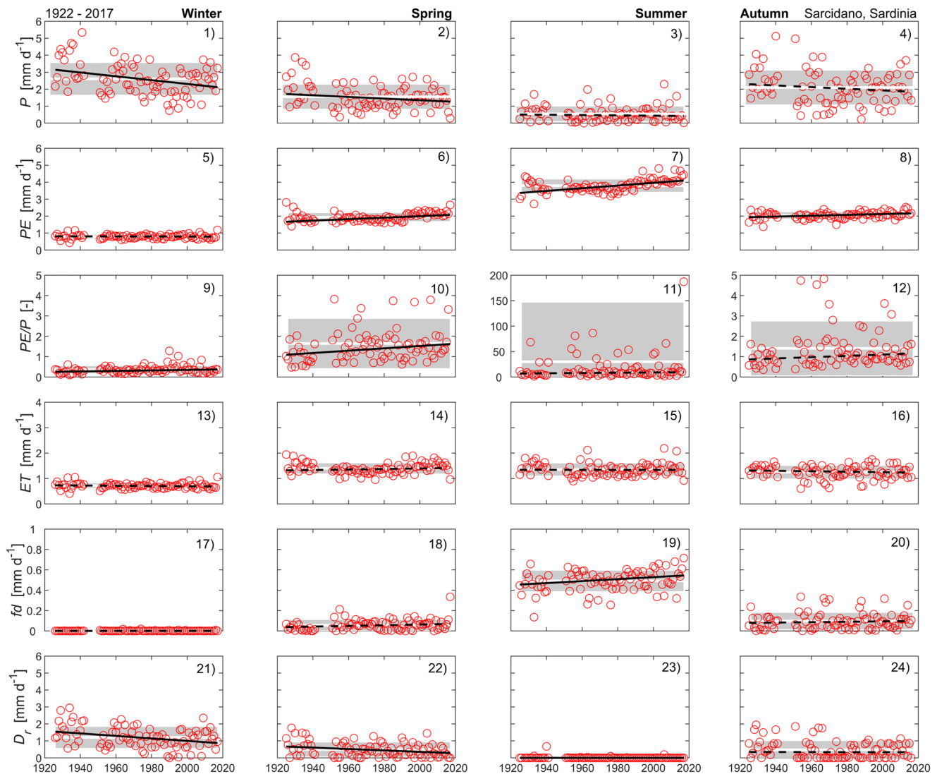
Figure 6. Historical seasonal, mean precipitation ( P ), potential evaporation ( PE ), index of dryness ( PE/P ) from two stations near Orroli in the area of Sarcidano, Sardinia, and predicted evapotranspiration ( ET ), vertical flux through the bottom of the soil layer ( f_d ), and drainage ( D_r ), represented by a white horizontal bar (mean) bracketed by gray bars (1 standard deviation). The trends using the Mann-Kendall approach are estimated with slopes from the Theil-Sen method (significant trends at p < 0.01 , are continuous black lines, while not significant are dashed black lines).
