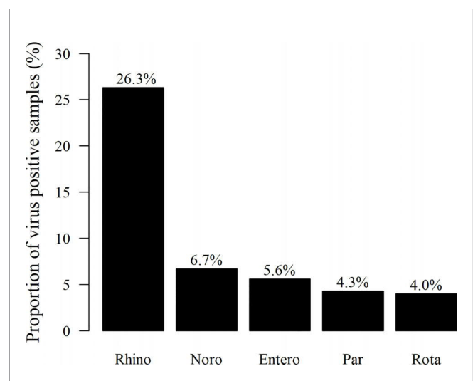
FIGURE 1 | Proportion (%) of stool samples positive for either enteral or respiratory viruses (433 samples) tested, from all 1,063 stool samples collected during the first 12 months of life. The most frequently detected virus was rhinovirus (Rhino) in 280 of the virus-positive samples, followed by norovirus G1/G2 (Noro) (71), enterovirus (Entero) (59), parechovirus (Par) (46), and rotavirus (Rota) (42 samples), respectively.
