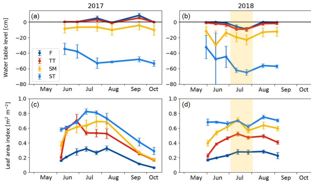
Figure 4. (a, b) Mean water table level and (c, d) average vascular leaf area index in the chamber plots in 2017 and 2018. F indicates flark, TT indicates Trichophorum tussock, SM indicates string margin, and ST indicates string top. Error bars represent the standard deviation within a plant community type. The drought period in July 2018 is denoted with shading.
