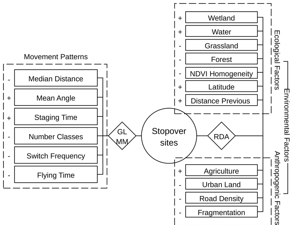
Fig. 1. A framework for the effects of human activities on waterfowl movements. GLMM = General Linear Mixed Model; RDA = Redundancy Analysis. A higher value of the movement patterns marked with “+” indicates a higher habitat quality with lower disturbance, while a higher value of those marked with “-” indicates a lower quality. The environmental factors marked with “+” were hypothesized to positively affect geese movement patterns related to high-quality habitats, while the ones marked with “-” were hypothesized to positively affect geese movement patterns related to low-quality habitats.
