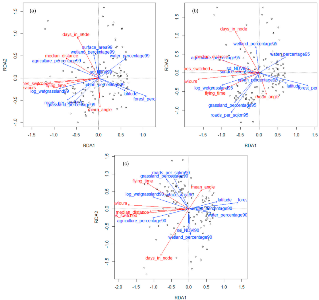
Fig. 4. Triplots from the three Redundancy Analyses (RDA) at the 99% (a), 95% (b), and 90% (c) area. The red arrows are movement variables, blue arrows represent environmental factors. The circles are sites. The first axis explained 11% of the variation at the 99% and 95% scale, and 12% at the 90% scale, and the second axis explained 6% of the variation at all scales.
