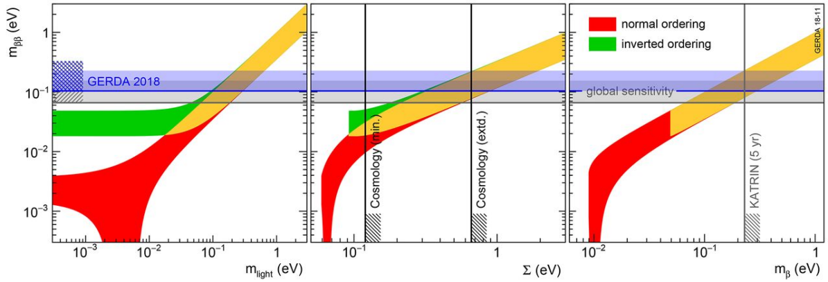
Figure 2. GERDA: Upper limit to the mass of the neutrino is 0.07 eV to 0.16 eV.
