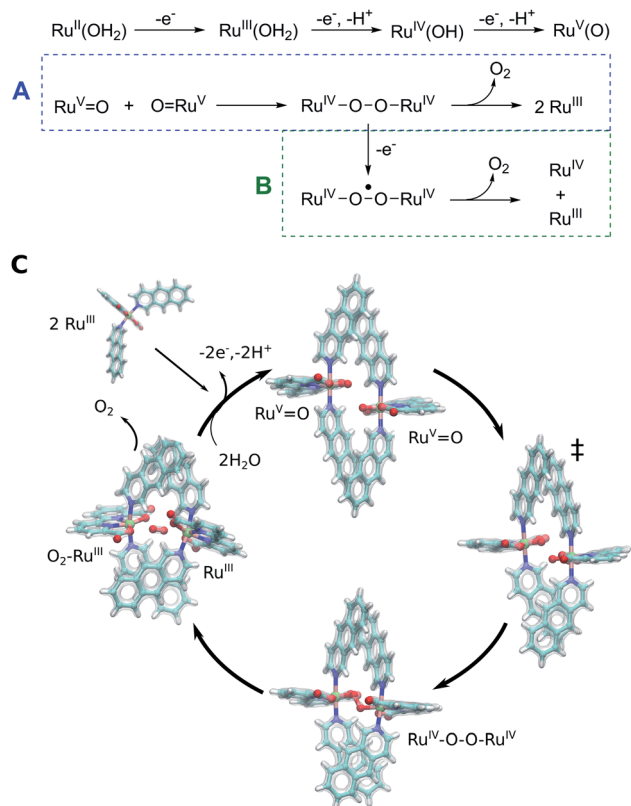
Fig. 5 Putative reaction mechanism of catalyst 3. Oxidation of Ru II -H 2 O yields the Ru V =O species from which the catalysis starts. Catalyst 3 forms a dimeric core complex, and via radical coupling and peroxy Ru IV -O-O-Ru IV intermediate yields O 2 (pathway A). Under highly oxidizing conditions, the Ru IV -O-O-Ru IV intermediate could be further oxidized to yield O 2 and a mixed valence Ru IV /Ru III product state (pathway B). (C) Structure of computed intermediates within putative reaction cycle of catalyst 3.
