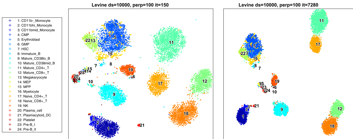
Fig. 2. Levine bone marrow data mapped into 2-D. Left panel: qSNE with rank-11 Hessian matrix approximation after only 150 quasi-Newton iterations; and right panel: t-SNE after 7280 iterations (cf. Fig. 1). The datasets were randomly downsampled to 10 000 samples and perplexity is set to 100 in both cases
