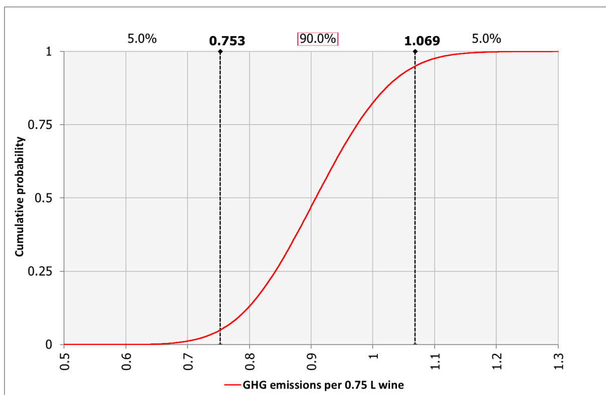
Figure 3: Monte Carlo simulation of GHG emissions per FU
