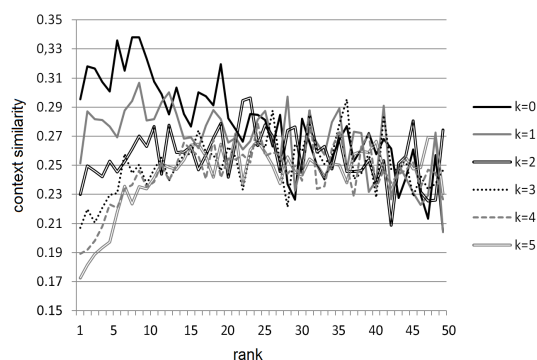
Figure 3: Rank-wise average context similarity.
