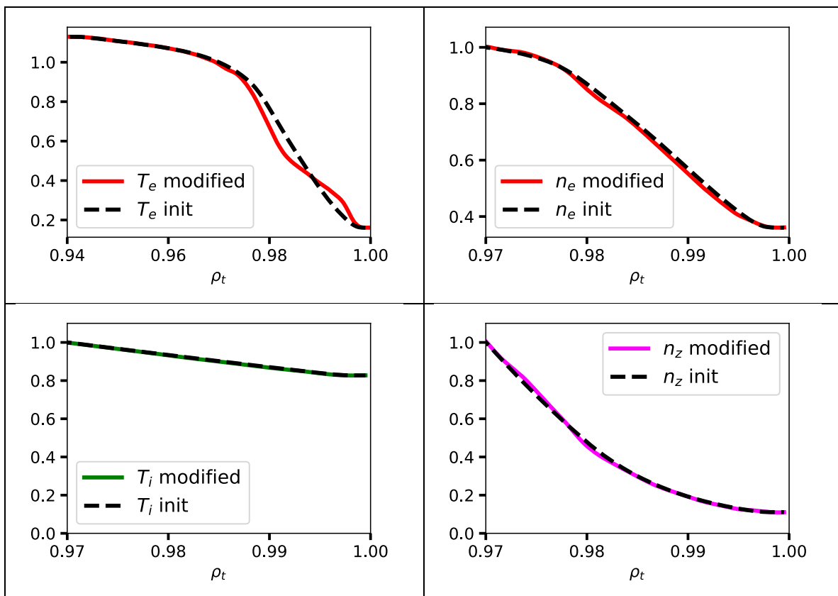
Figure 17: Profile modifications in nonlinear MTM simulations. Shown is case, mod5 n=15 . Only the T_e profile is significantly affected, consistent with the inter-ELM profile evolution observed experimentally on shot 153674/5. Nonlinearly modified profiles in the saturated state (solid line) are compared to the initial profiles (dashed line).
