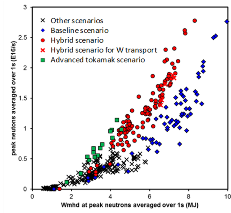
Figure 2. Neutron rate as function of plasma stored energy achieved at JET in 2016 campaigns in baseline and hybrid plasmas and in plasmas optimized for alpha particle studies.
