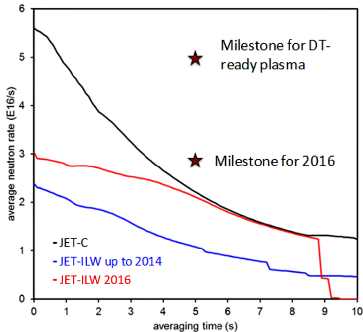
Figure 1. Average D-D neutron rate as function of the averaging time for JET's best performing shots. The stars show the milestones for 2016 and a for a D-T ready plasma.
