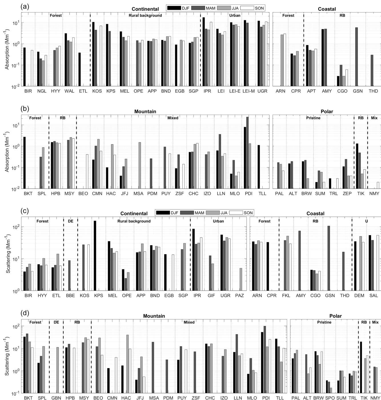
Figure 6. Variation of the seasonal median of absorption coefficient ( a , b ) and scattering coefficient ( c , d ) for the different sites, grouped according to site classification of Table 3 with DE (Desert), U (Urban), and RB (Rural Background).
