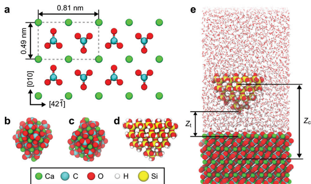
Fig. 1 Atomistic models of the calcite ( 10\bar{1}4 ) surface and the tip used for the simulations. (a) Calcite ( 10\bar{1}4 ) surface. (b) Ca tip. (c) \text{CO}_3 tip. (d) OH tip. (e) Snapshot of the simulation model including the tip, sample (calcite) and water. z_t is defined as the vertical distance between the tip apex atom and the surface Ca atom.
