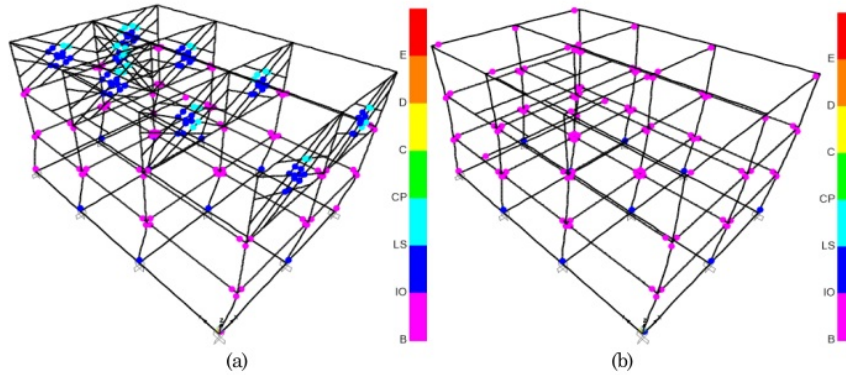
Figure 7. Damages of Three-Story RC Building in Final Step t=50s for Scheme 1 Design Earthquake Level: (a) FIX-INF, (b) FIX-LOAD
