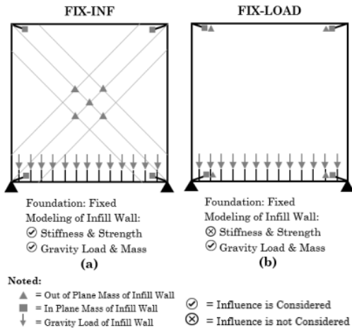
Figure 4. Variation Model Based on Fixed Foundation
