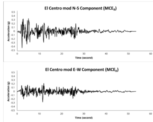
Figure 6. Modified El Centro 1940 (El Centro Mod) Accelerogram N-S and E-W Direction
