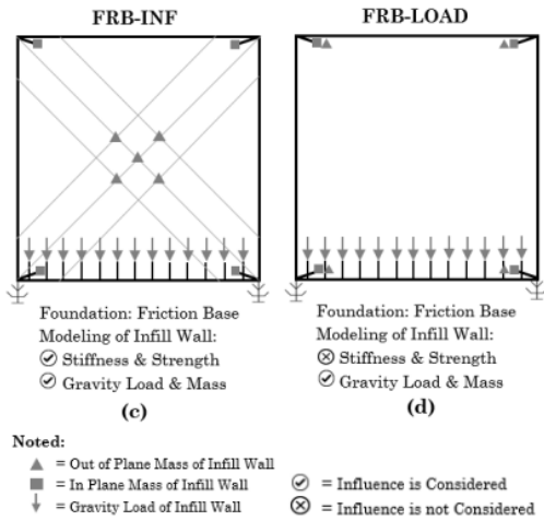
Figure 5. Variation Model Based on Friction Base Foundation
