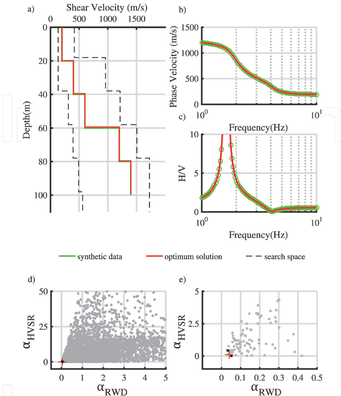
Figure 10. Results for SM-2. Synthetic model and a model obtained from the Pareto optimum particle and the parameter search space (a); the fit between the observed and calculated RWD (b), and HVSr (c); the Pareto optimum solution marked as + and Pareto front (dark dots) with the dominated particles (light dots) for all iterations (d); and the Pareto optimum solution (+) with Pareto front and dominated particles at the last iteration (e) [8].
