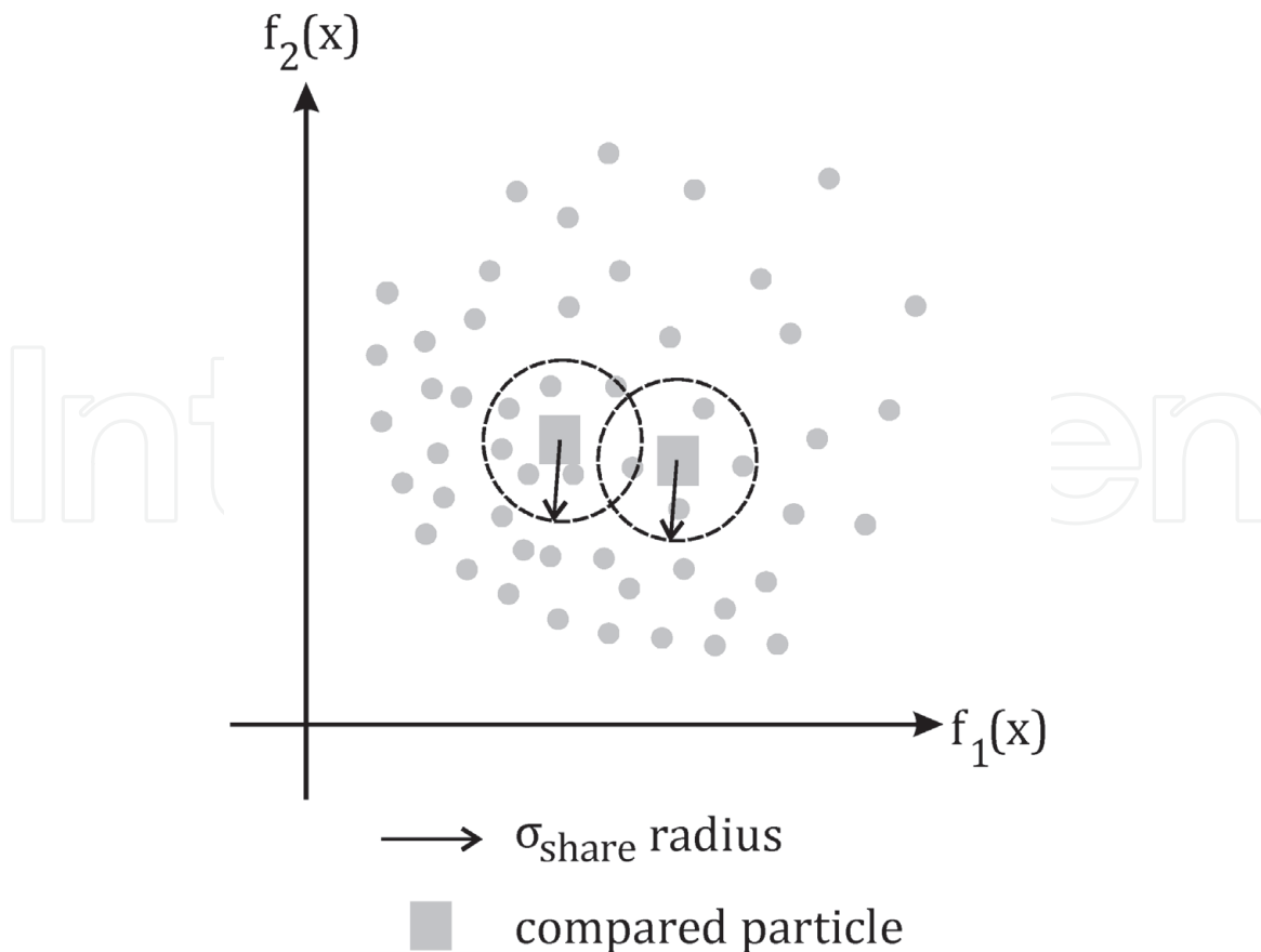
Figure 6. Niches having radius indicated by \sigma_{share} are generated to compare of particles that have not change after several iterations.
