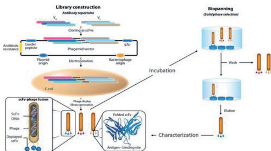
Figure 5. Phage display method to build library of peptides and proteins variants (source: Almagro et al. [62]).
