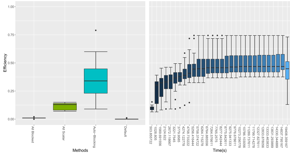
Figure 3: MCMC efficiencies of different methods for spatial model. The left panel shows the box-plots of MCMC efficiencies of All Blocked, All Scalar, Auto Block and Default algorithms computed from 20 replications. The right panel shows the box-plots of MCMC efficiencies of Nested Adaptation 5K algorithm computed from 20 replications at each outer adaptation. The last (right-most) box-plot is computed from the chain of 10000 samples generated. The time axis shows the average computational time of 20 replications.
