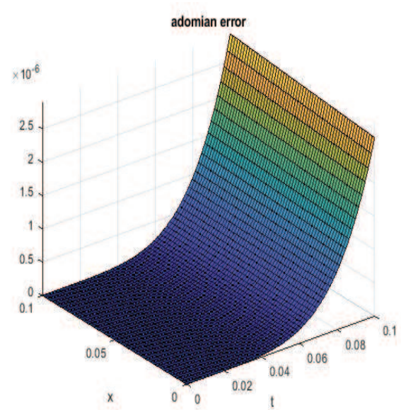
Fig. 1: The difference between the exact solution and the solution with Adomian polynomial of u_{xx} = u_{tt} + 2u_t + u^2 - e^{(2x-4t)} + e^{(x-2t)} .
