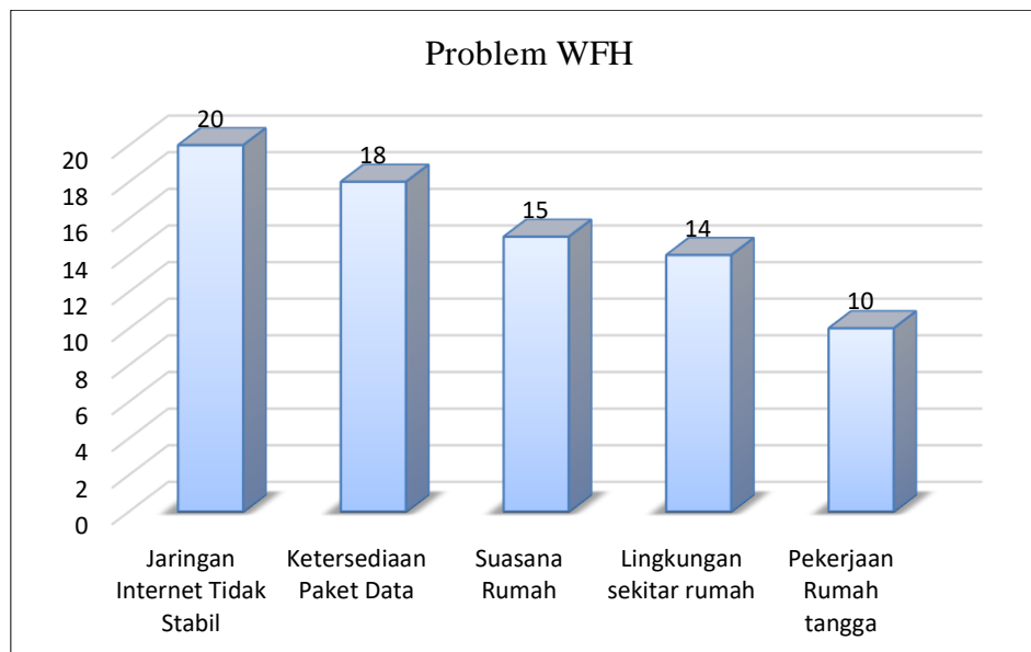
Gambar 2. Problem WFH
