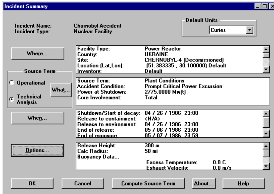
Figure 16. Incident Summary Window
