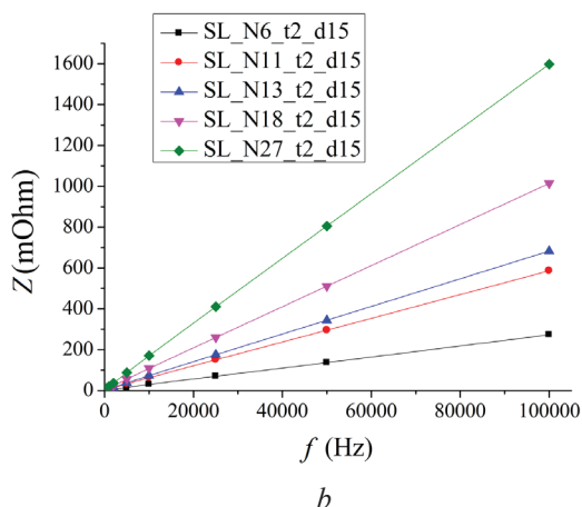
Figure 3 – Graphs of the dependence of the total resistance of single-layer coils on the current frequency: a – coil diameter 7 mm; b – coil diameter 15 mm
