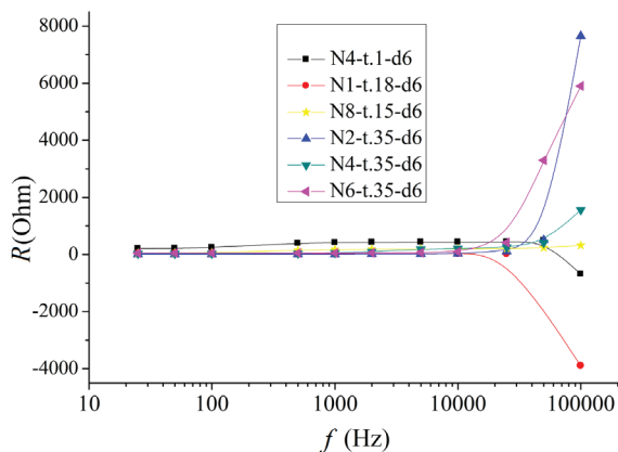
Figure 5 – Dependence of the resistance of multilayer coils on the frequency of the current
