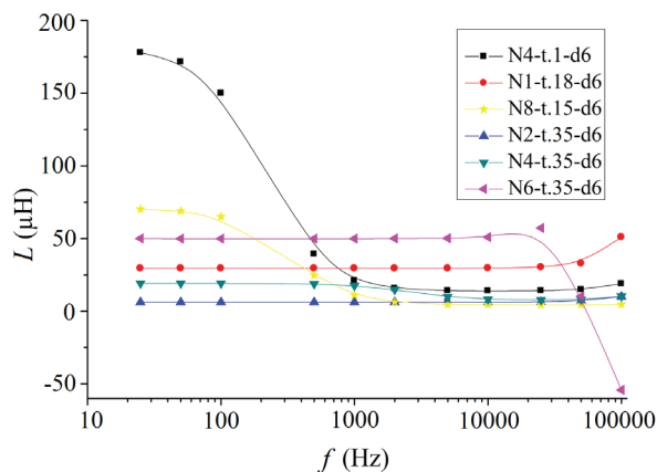
Figure 4 – Graph of the dependence of the inductance of multilayer coils on the current frequency
