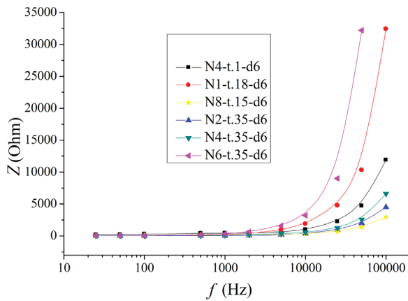
Figure 6 – Dependence of the total resistance of multilayer coils on the frequency of the current
