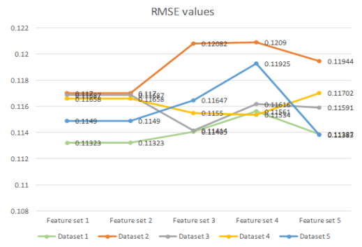
Fig. 10. Line graph of comparison between all datasets using every significant feature set
