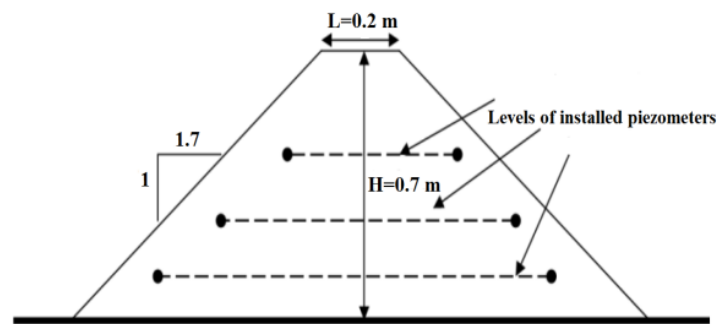
Figure 1. Geometry and specification of the experimental model
