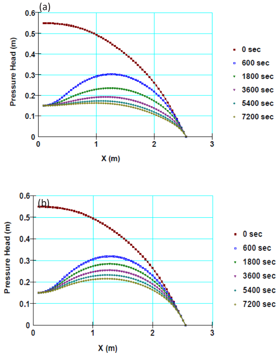
Figure 14. Changes in pore water pressure inside the dam body based on conductivity Constant saturated hydrocarbon (a) and unsaturated hydraulic conductivity (b).
