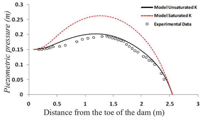
Figure 15. Piezometric pressure in non-permanent leak analysis 30 minutes after the drop in the reservoir's water level from a level of 60 to 15 cm in a piezometer: First row (lowest row).
