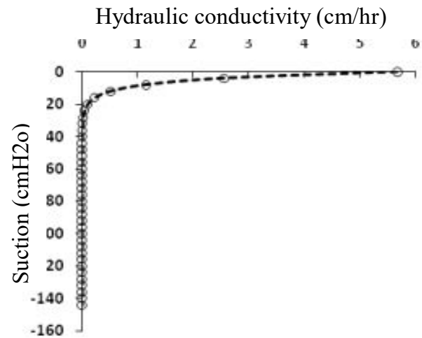
Figure 6. Variation of the permeability of the materials in different suctions
