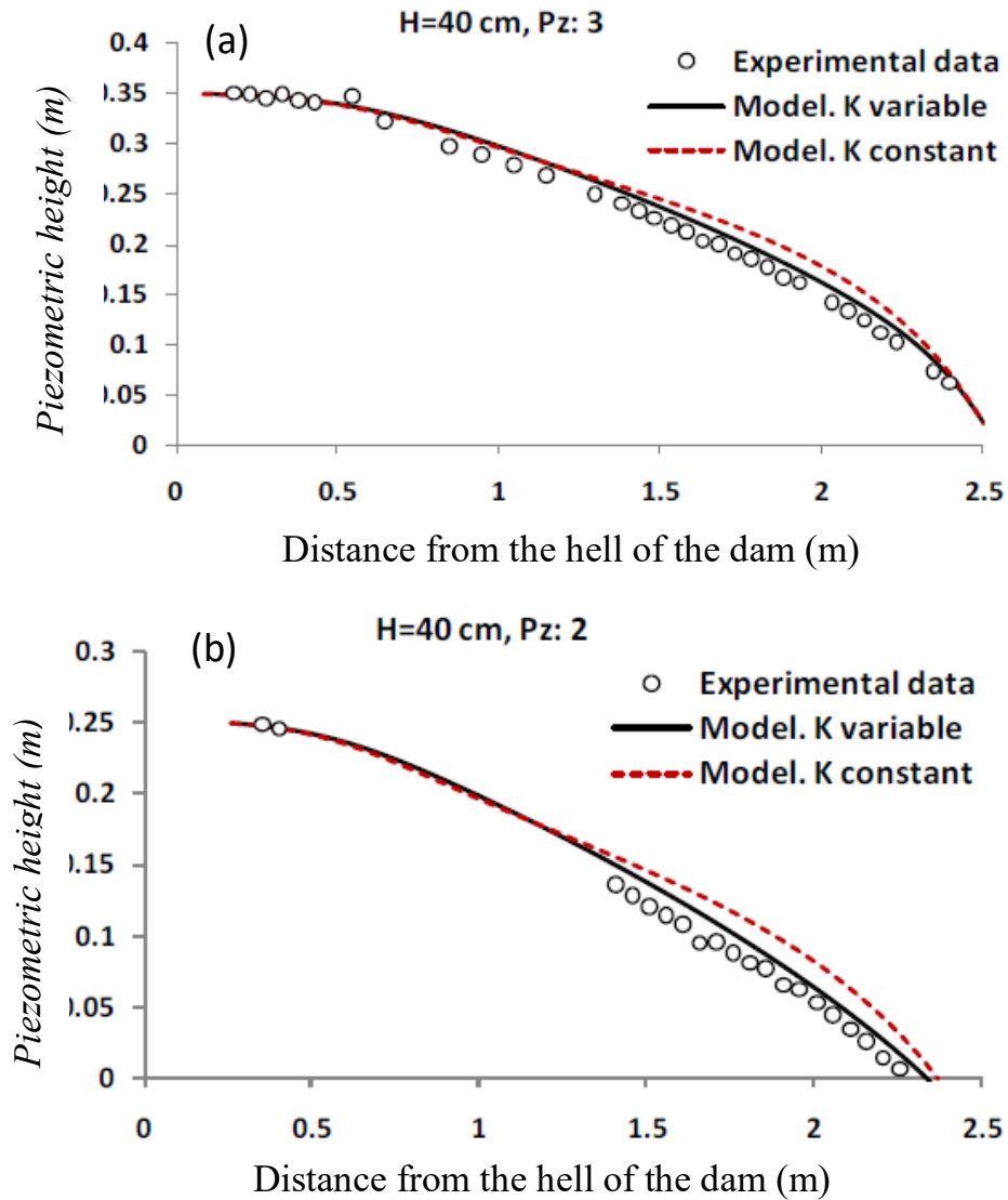
Figure 10. Comparison of the pressure load in the piezoelectric cells of the first (a) and second (b) row. Laboratory data with saturated and unsaturated hydraulic conductivity in the state reservoir water level of 40 cm.
