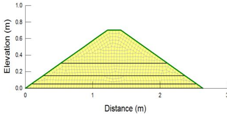
Figure 7. A view of mesh used based on triangular and quad elements.
