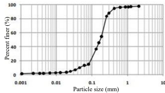
Figure 3. Grain size distribution of the dam body
