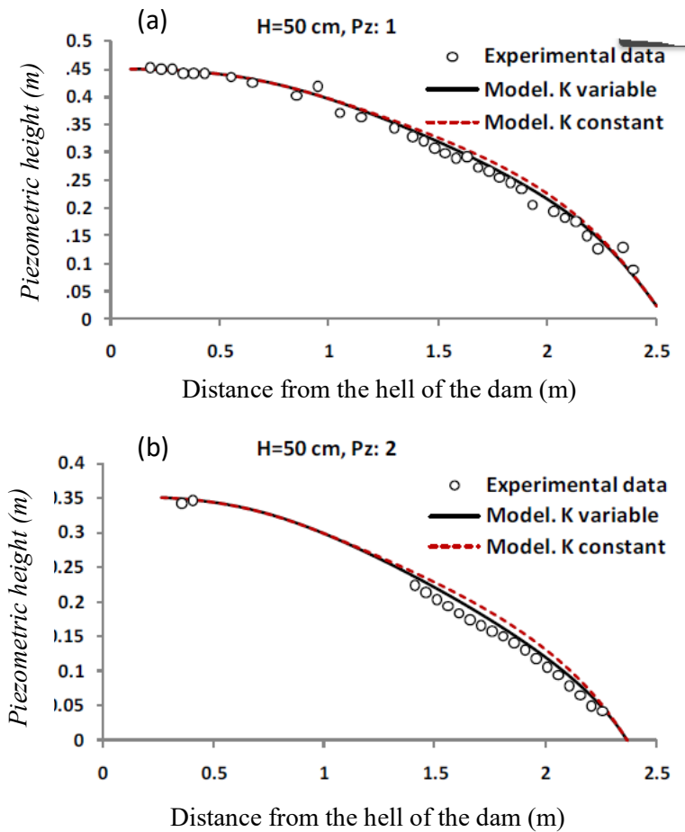
Figure 9. Comparison of pressure load in first (a) and second (b) row piezoelectric sensors with experimental data with saturated and unsaturated hydraulic conductivity in the state reservoir water level of 50 cm.
