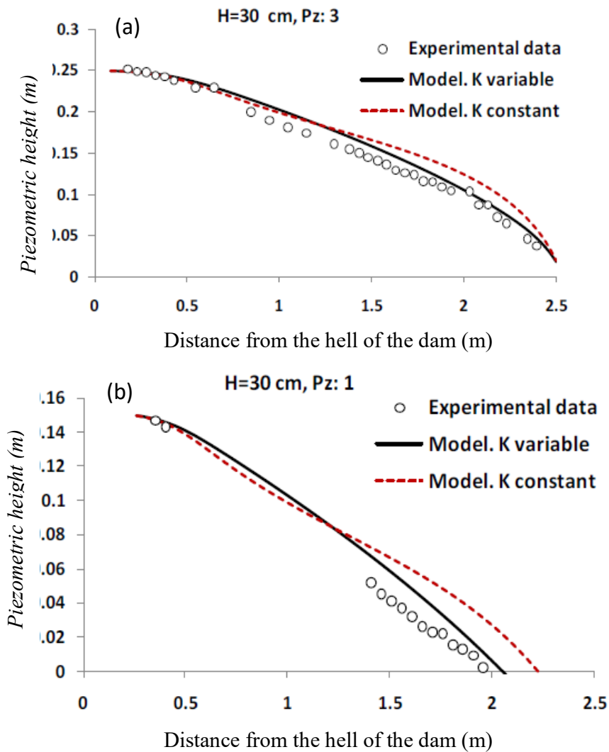
Figure 11. Comparison of the pressure load in the piezoelectric cells of the first row (a) and second row (b). Laboratory data with saturated and unsaturated hydraulic conductivity in the state reservoir water level of 30 cm.
