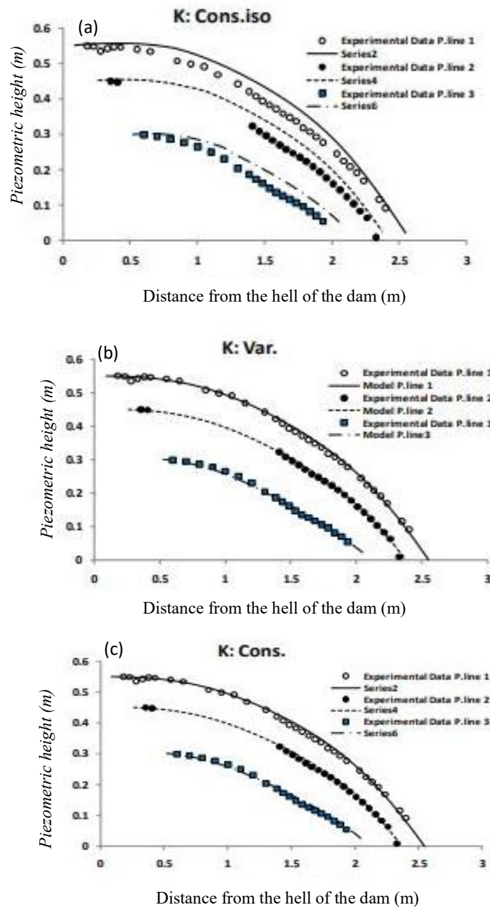
Figure 8. Comparison of measured piezometric data and modeled results. Note: Prior to calibration, using a saturated hydraulic conductivity of Penetration experiments on the soil sample are also considered (a) and after calibration based on three rows of piezometers installed in the laboratory model and non-hydraulic conductivity Saturation (b) and saturation (c) in a non-coercive state.
