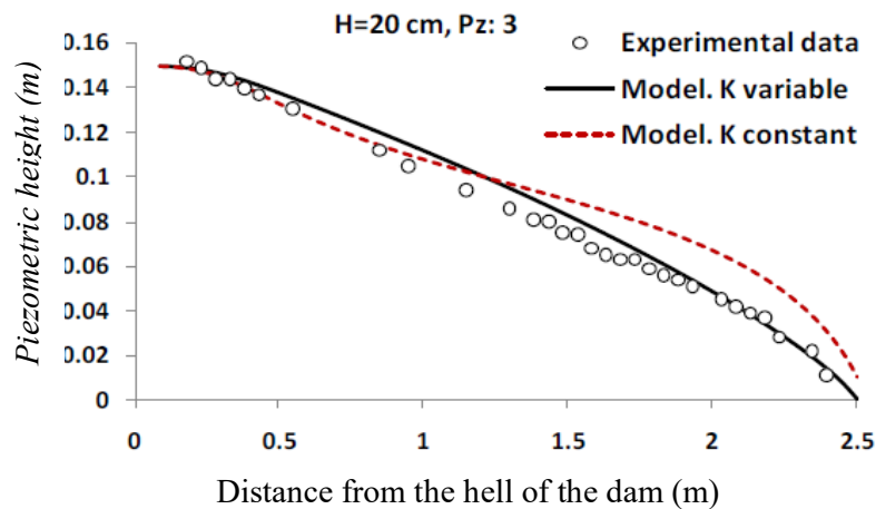
Figure 12. Comparison of pressure load in third row piezoelectric sensors with laboratory data with saturated and unsaturated hydraulic conductivity in the state reservoir water level of 20 cm.
