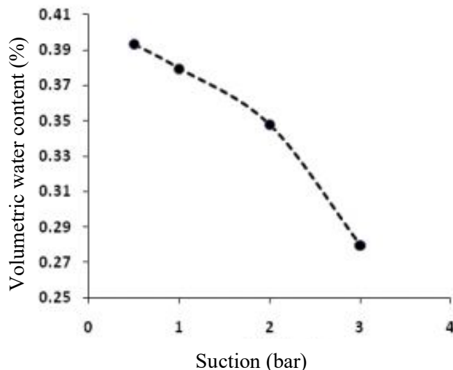
Figure 4. Moisture characteristic curve of the body materials of the experimental model homogeneous dam
