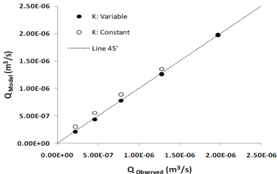
Figure 13. Comparison of leakage values from numerical analysis in two different conditions. Application of constant saturated hydraulic conductivity and hydraulic conductivity variable with leakage values observed.
