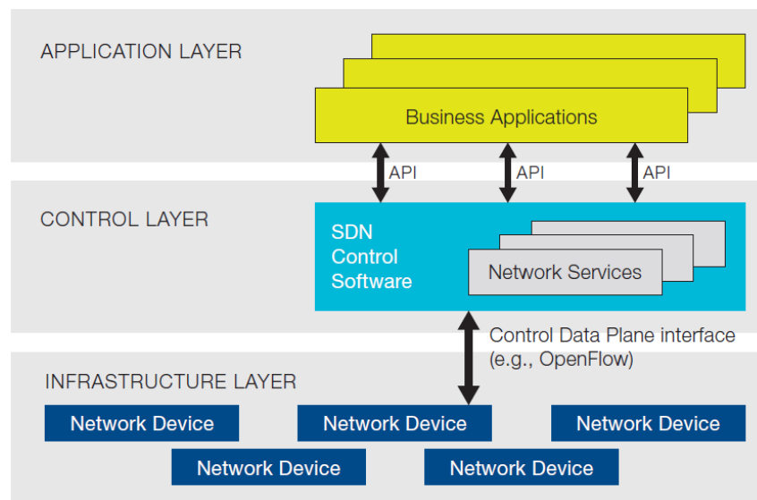
Figure 4: Software-Defined Network Architecture. (source: opennetworking.org )
