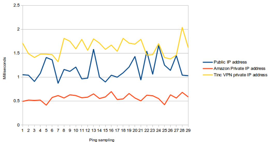
Figure 8: Tinc evaluation: Graph showing different ping times in milliseconds for a period of 30 seconds
