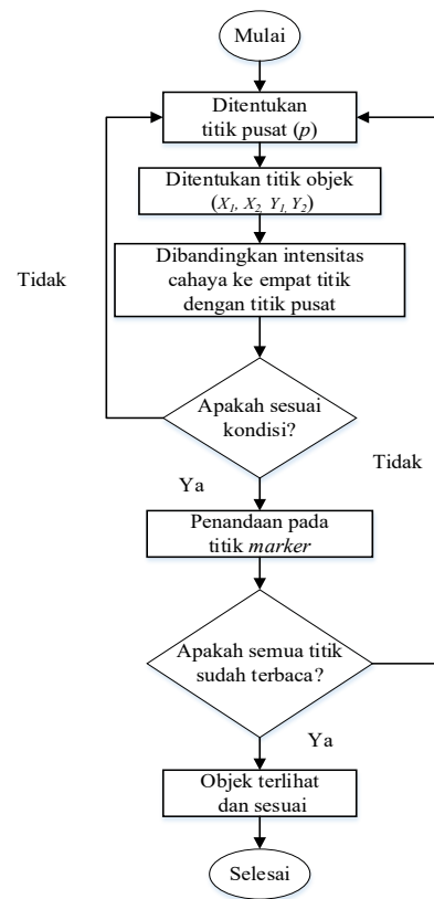
Gambar 5. Diagram Alir FAST corner detection
