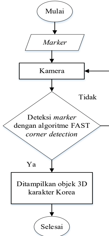
Gambar 3. Diagram Alir Pendeteksian Marker
